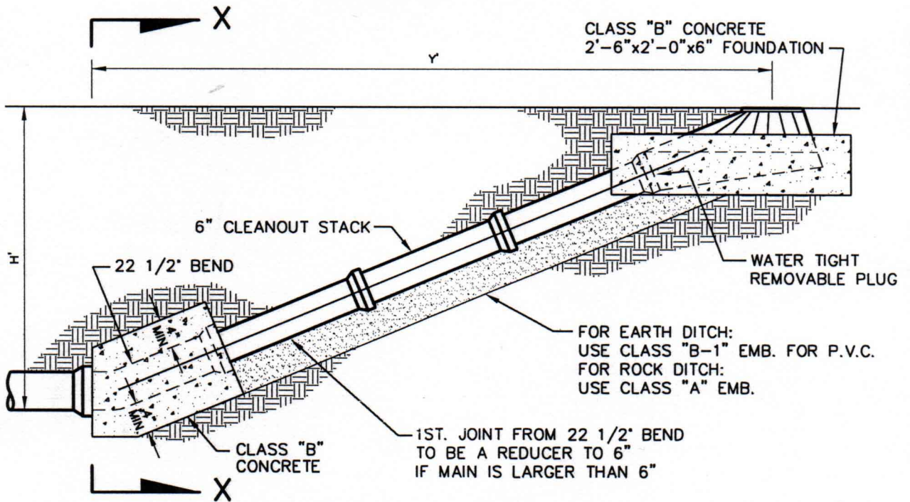
PROFILE VIEW
